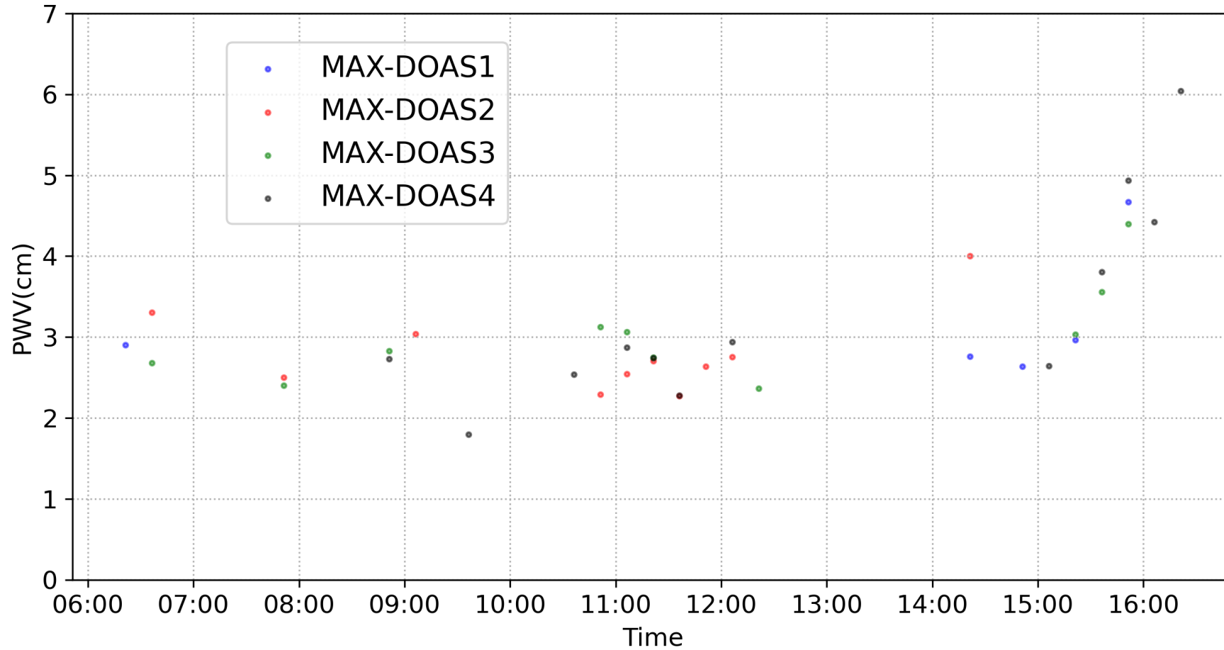
PWV(cm) of MAXDOAS1-4 in Chiba 2021/08/08
