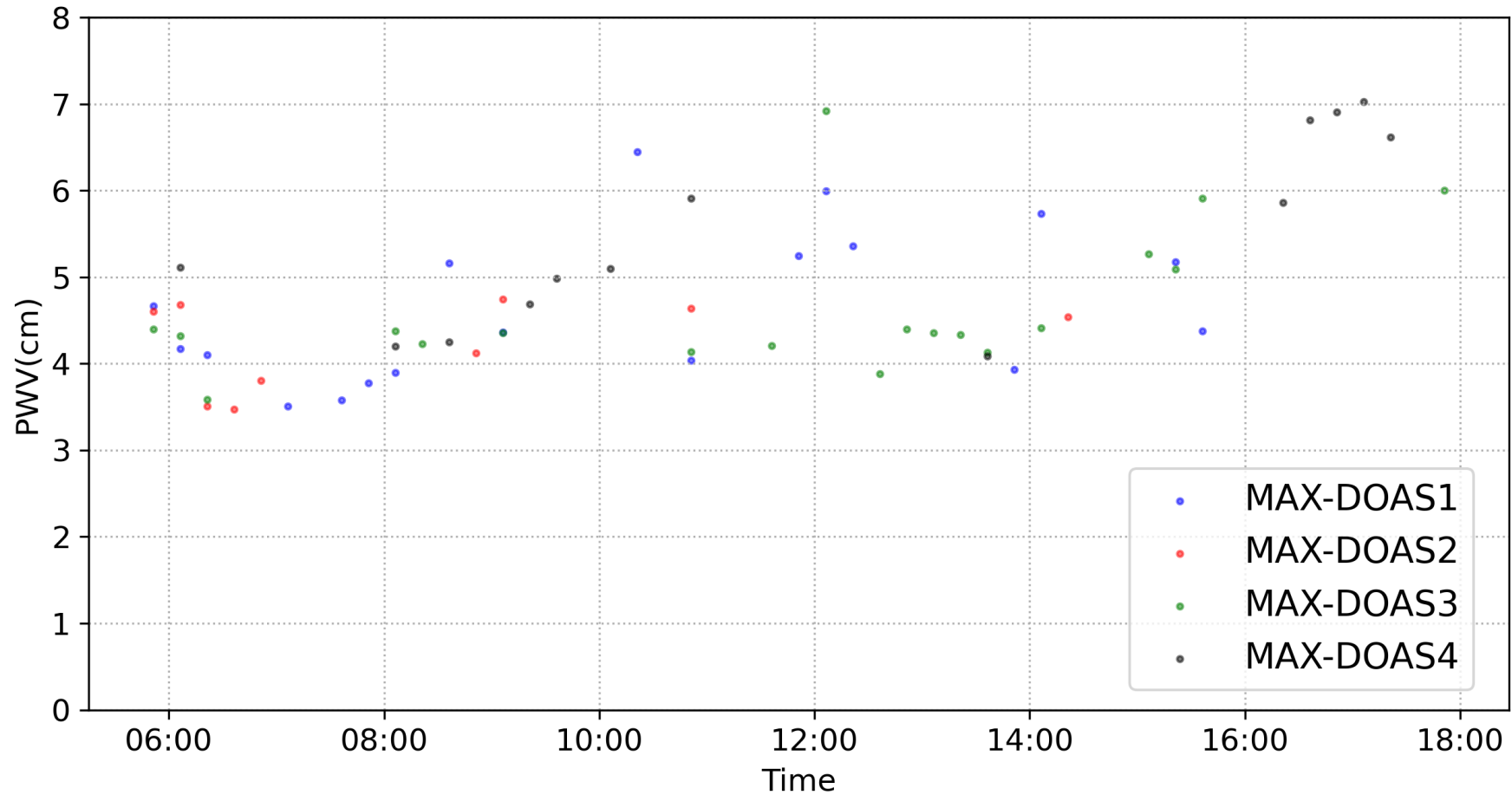
PWV(cm) of MAXDOAS1-4 in Chiba 2021/08/07
